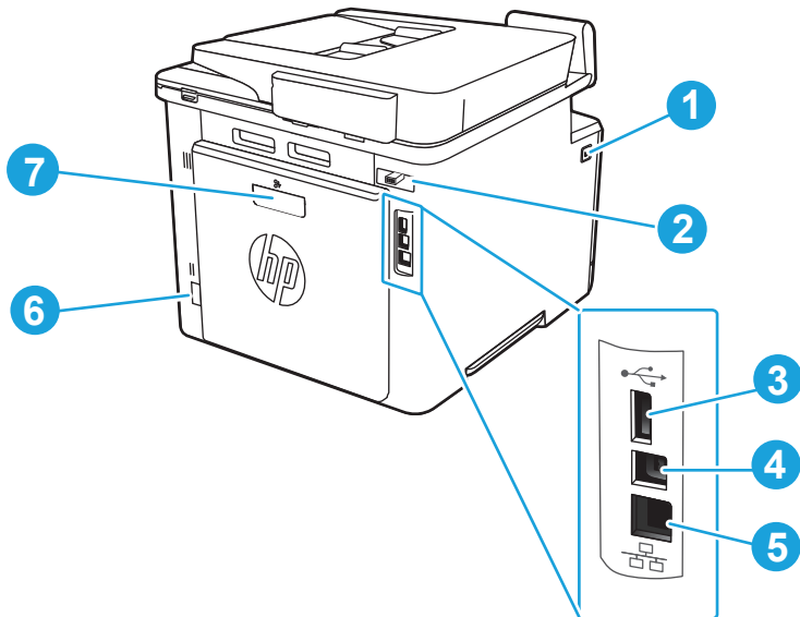
Figure 1-7 Printer rear view
