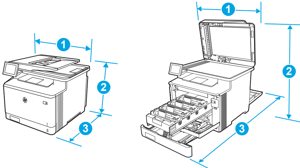
Figure 1-9 Dimensions for the E47528f model
