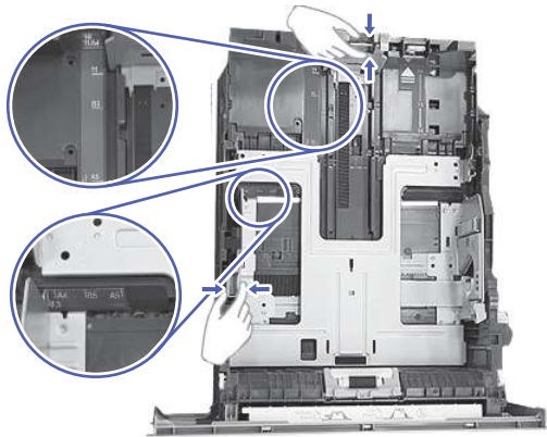
Figure 9-17 Adjust guides
