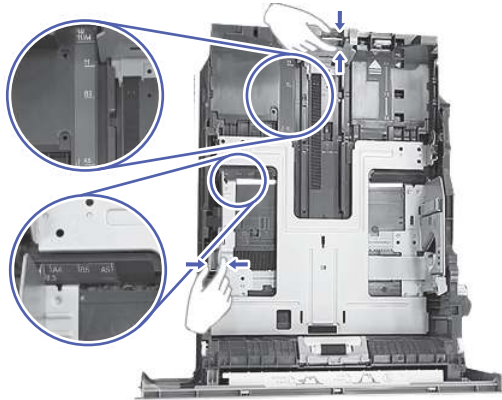
Figure 9-20 Adjust guides
