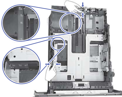
Figure 9-16 Adjust guides
