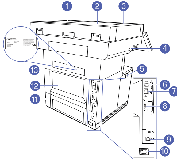
Figure 1-9 Printer rear view - 6600, 6600dn and 6600zfw models
