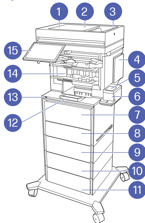
Figure 1-8 Printer front view - 6600zfs
