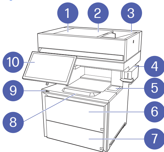
Figure 1-7 Printer front view - 6600zfw
