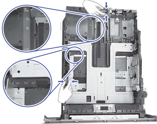
Figure 9-18 Adjust guides
