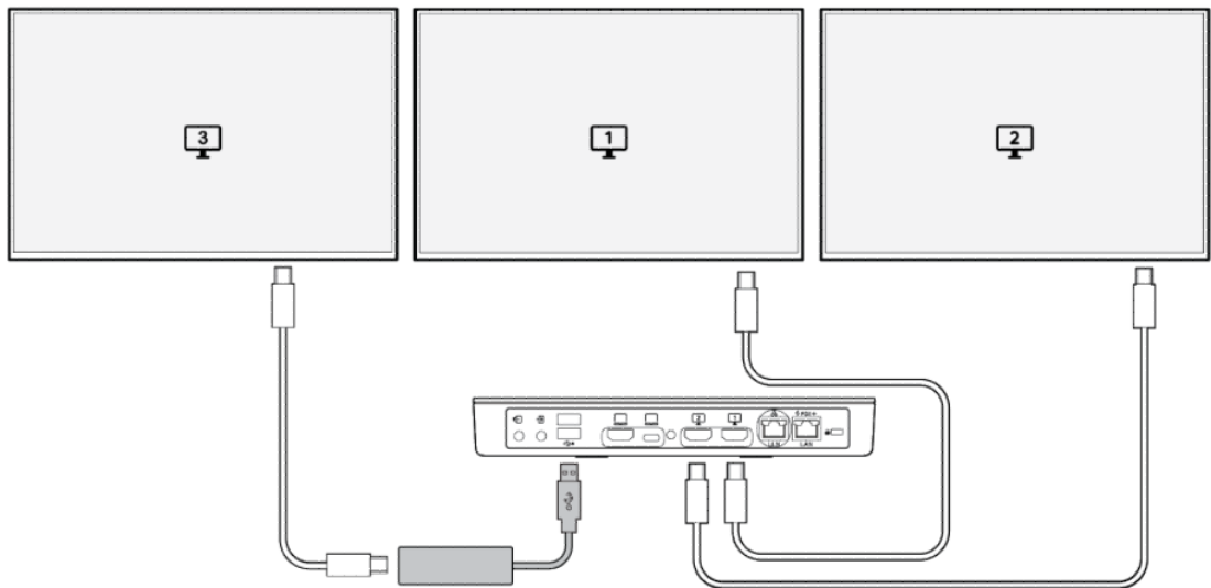
Figure 12-1 Poly Studio G62 with a Pluggable USB to HDMI adapter with a third monitor connected
