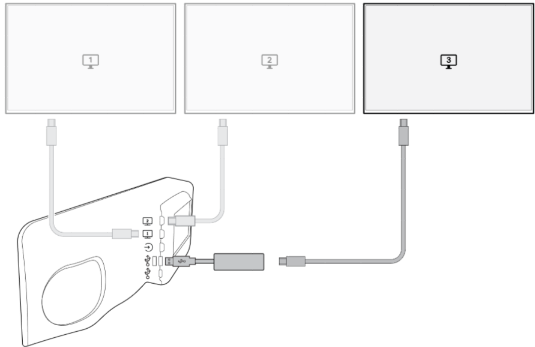
Figure 12-2 Poly Studio X72 with a Plugable USB to HDMI adapter with a third monitor connected
