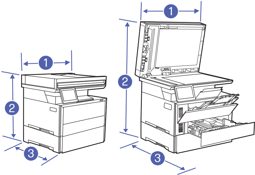
Figure 1-10 Dimensions for the printer with the optional 550-sheet tray
