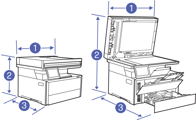
Figure 1-9 Printer dimensions
